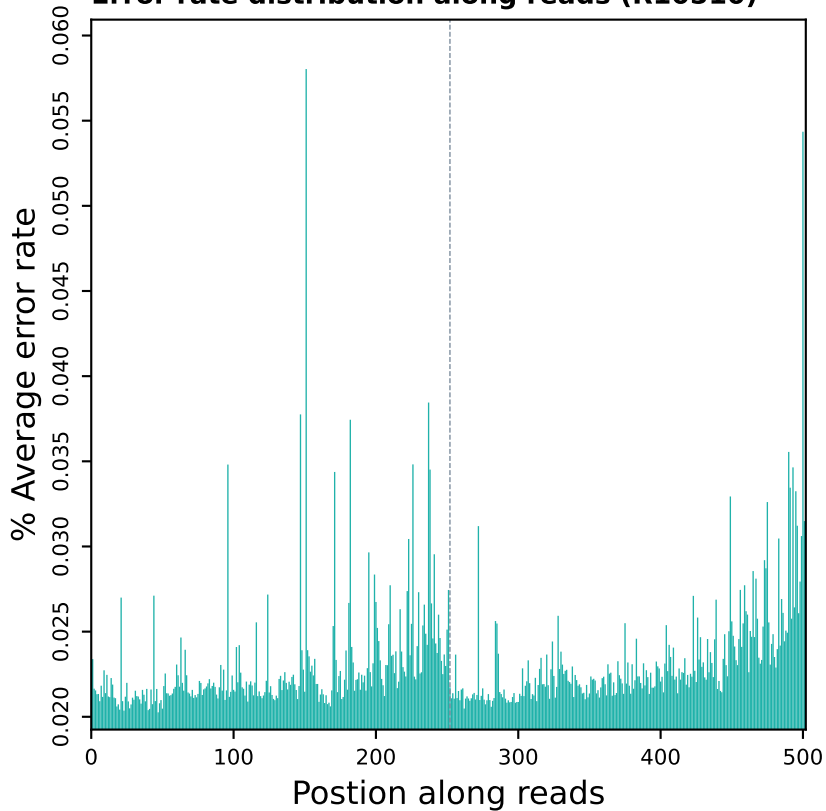
Error rate distribution along reads (R10510)
